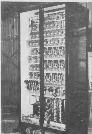
This is the controller for the new lift in the machine room on the 16th floor of the PCAR.
